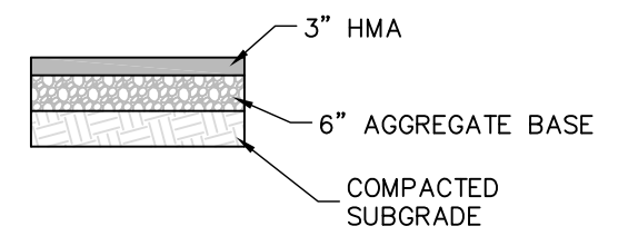
PAVEMENT SECTION
