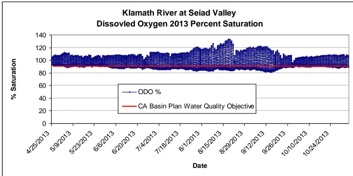
Figure 7. Percent saturation dissolved oxygen readings recorded every 30-minutes for Klamath River at Seiad Valley (SV) in 2013. The red line indicates the NCRWQCB Basin Plan Klamath River site specific dissolved oxygen water quality objective: from the mouth of the Scott River to Hoopa, >90% saturation year-round.
