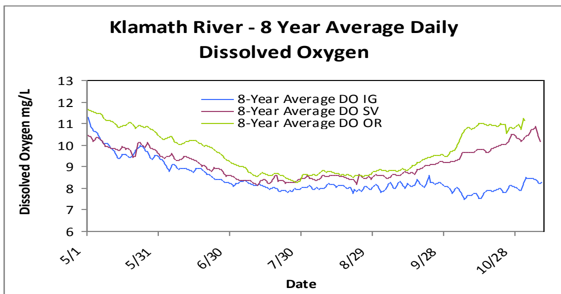
Figure 9. Average daily dissolved oxygen levels from 2006-2013 at mainstem Klamath River sites: below Iron Gate dam (IG), Seiad Valley (SV), and Orleans (OR).
