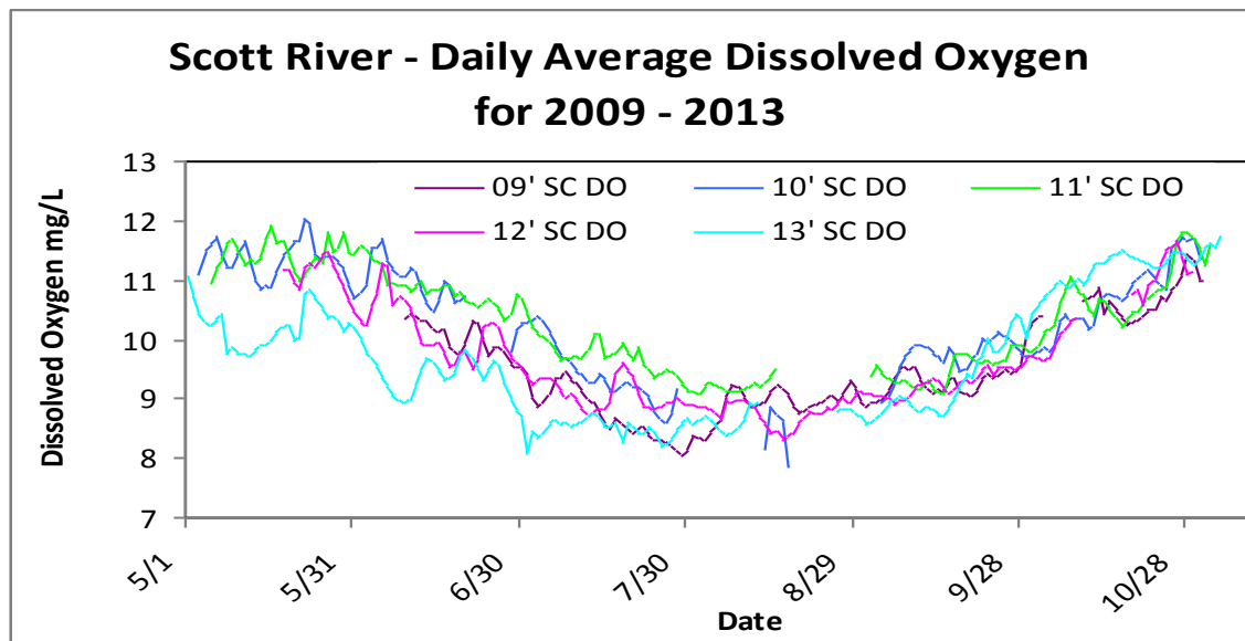
Figure 22. Daily average dissolved oxygen concentrations for the Scott River from 2009-2013.
