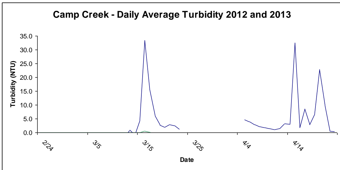
Figure 33. Daily average turbidity, winter of 2012 and 2013 on Camp Creek.
