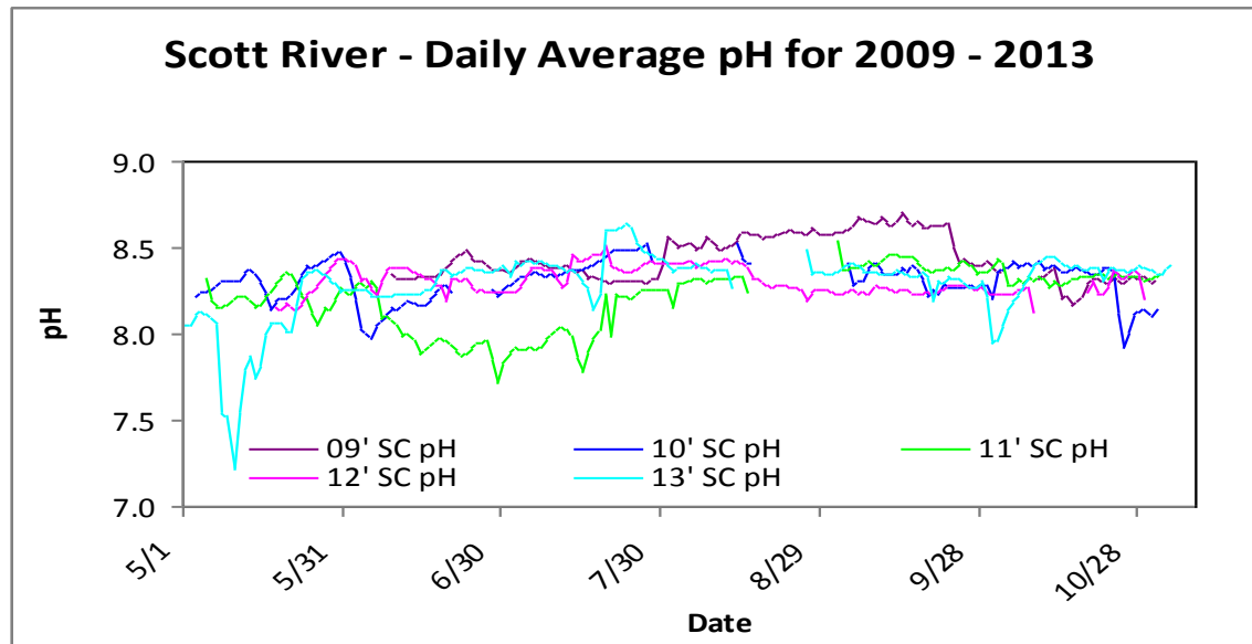
Figure 29. Daily average pH concentrations for the Scott River from 2009-2013.
