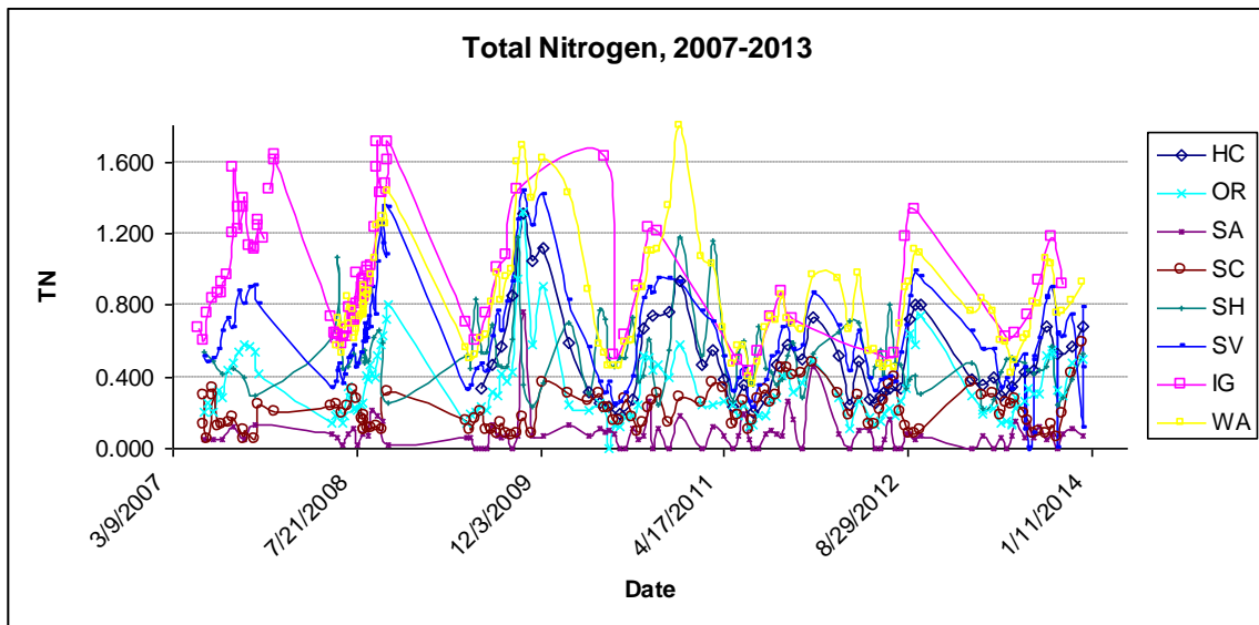
Figure 38. Total Nitrogen measured in mg/L for all monitored sites during 2007-2013.
