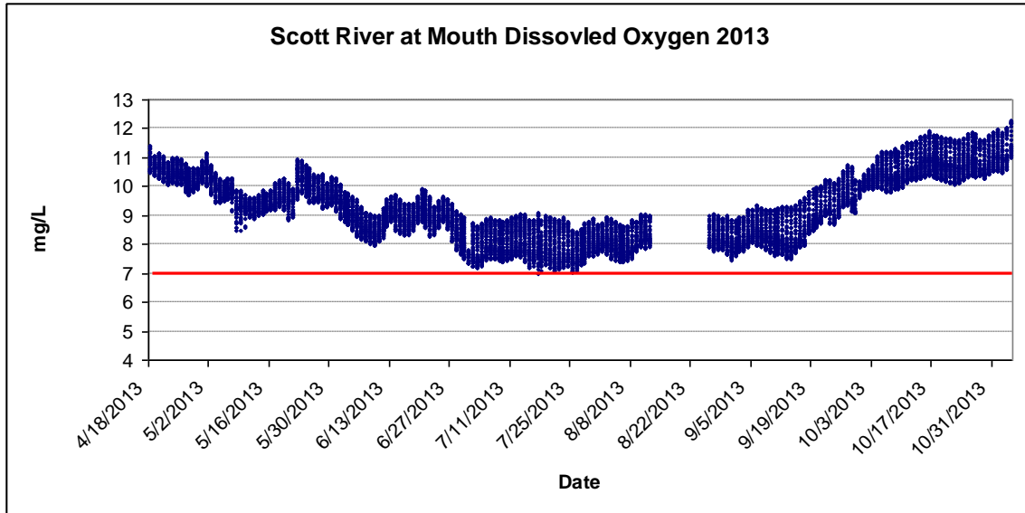
Figure 23. Instantaneous dissolved oxygen readings recorded every 30-minutes for the mouth of the Scott River (SC) in 2013. The red line indicates the NCRWQCB Basin Plan site specific dissolved oxygen water quality objective for Scott River, >7mg/L.
