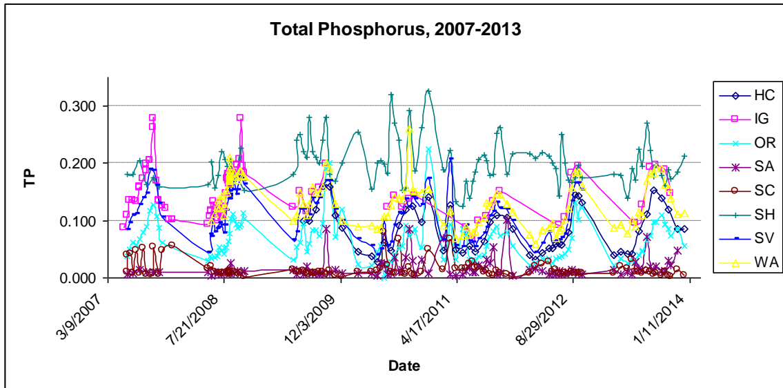
Figure 36. Total Phosphorus measured in mg/L for all monitored sites during 2007-2013.
