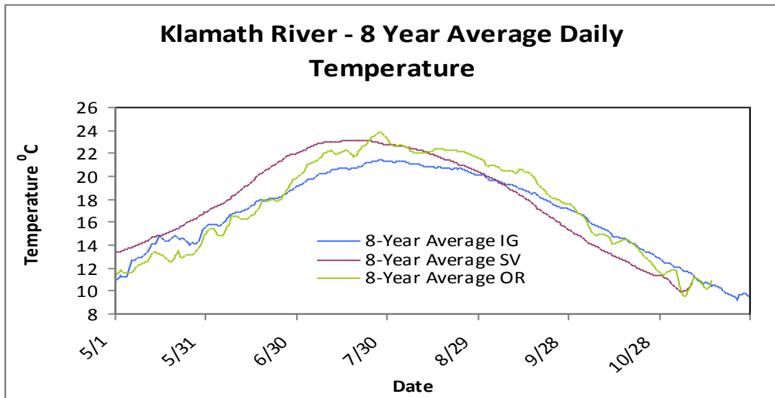
Figure 4. Averaged daily temperature from 2006-2013 at mainstem Klamath River sites: below Iron Gate dam (IG), Seiad Valley (SV), and Orleans (OR).
