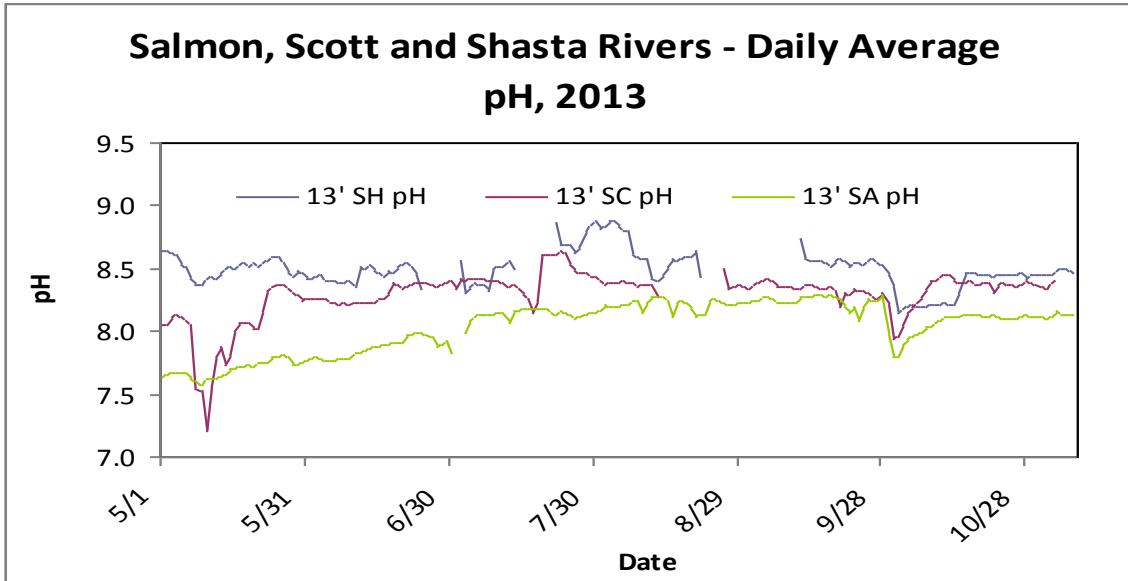
Figure 26. Daily average pH for Scott, Shasta, and Salmon Rivers, 2013.
