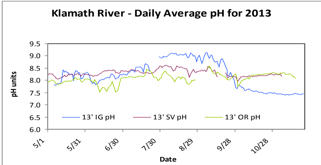
Figure 10. Daily average pH levels for 3 mainstem Klamath River sites in 2013: below Iron Gate dam (IG), Seiad Valley (SV), and Orleans (OR).
