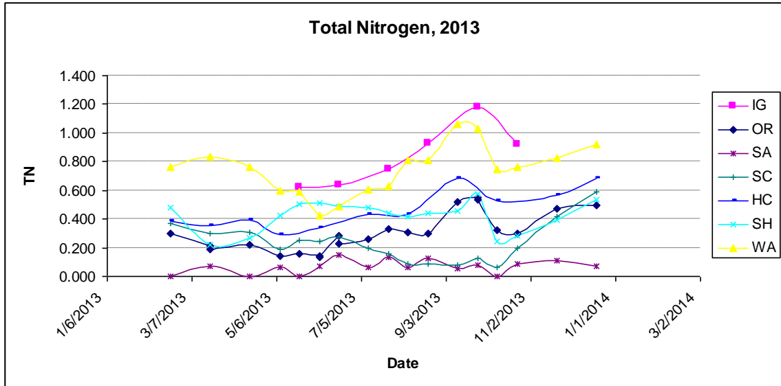
Figure 37. Total Nitrogen measured in mg/L for all monitored sites during 2013.
