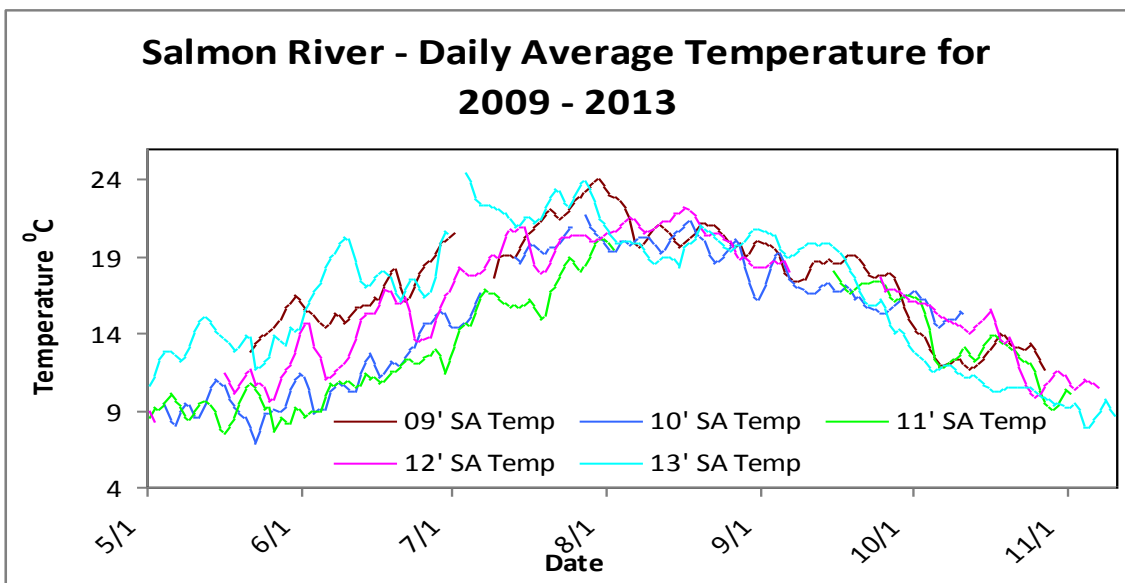
Figure 18. Daily average water temperatures for the Salmon River from 2009-2013.
