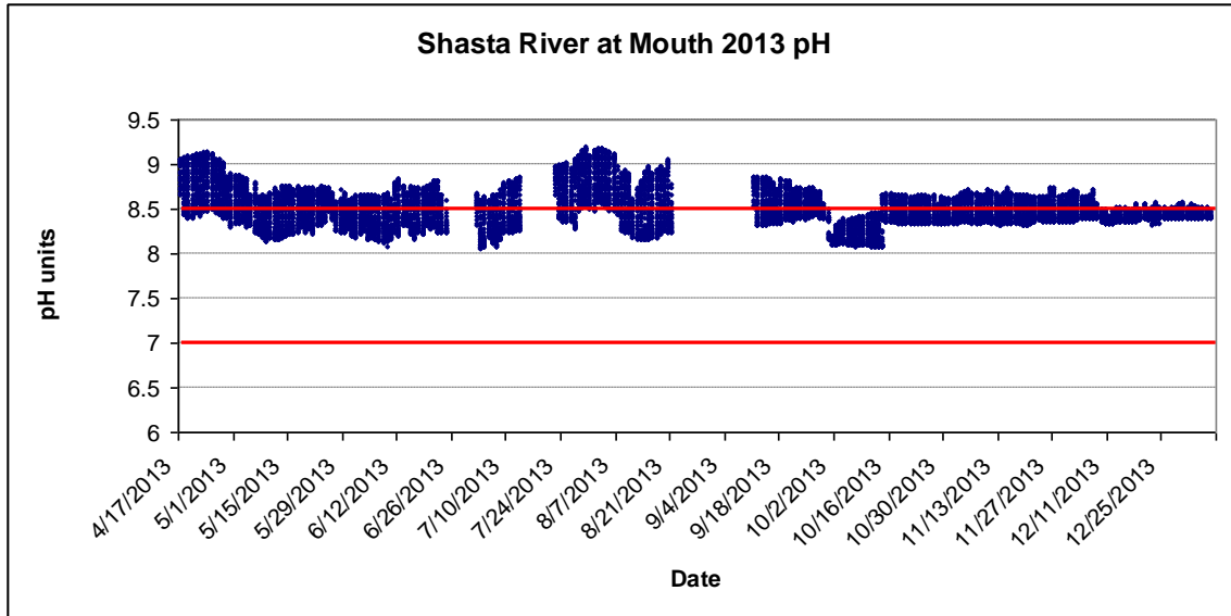
Figure 28. Instantaneous pH readings recorded every 30 minutes for the mouth of the Shasta River (SH) in 2013. The red line indicates the NCRWQCB Basin Plan pH water quality objective for Shasta River, 7 < X < 8.5 .
