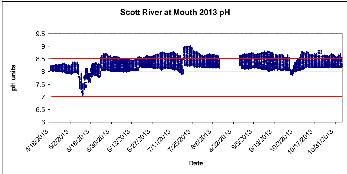
Figure 30. Instantaneous pH readings recorded every 30 minutes for the mouth of the Scott River (SC) in 2013. The red line indicates the NCRWQCB Basin Plan pH water quality objective for Scott River, 7 < X < 8.5 .
