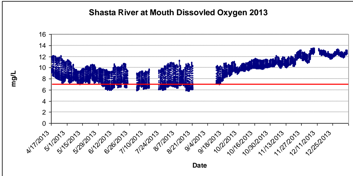
Figure 21. Instantaneous dissolved oxygen recorded every 30-minutes for the mouth of the Shasta River (SH) in 2013. The red line indicates the NCRWQCB Basin Plan site specific dissolved oxygen water quality objective for Shasta River, >7mg/L.
