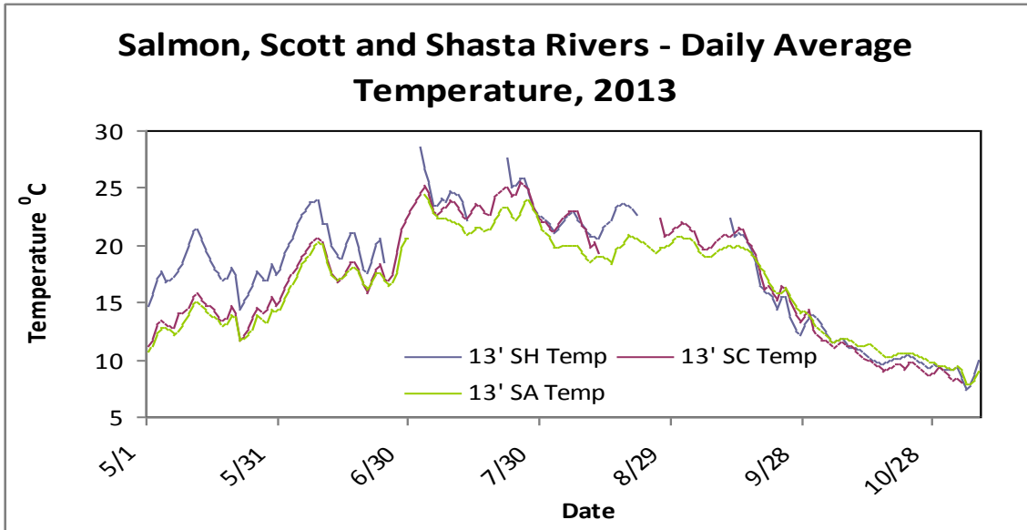
Figure 15. Daily average water temperature for Scott, Shasta, and Salmon Rivers, 2013.
