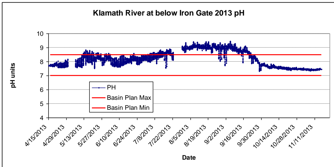
Figure 13. Instantaneous pH readings recorded every 30-minutes for Klamath River below Iron Gate (IG) in 2013. The red lines are the NCRWQCB Basin Plan water quality objectives for the Klamath River, 7 < X < 8.5
