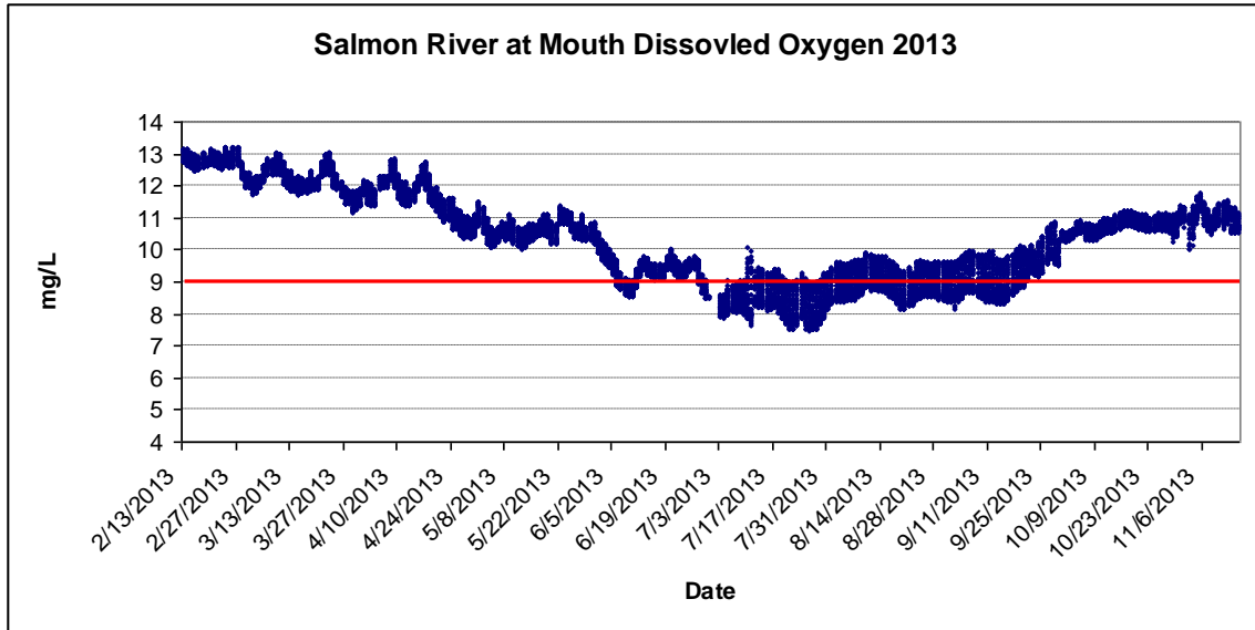
Figure 25: Instantaneous dissolved oxygen readings recorded every 30 minutes for the mouth of the Salmon River (SA) in 2013. The red line indicates the NCRWQCB Basin Plan site specific dissolved oxygen water quality objective for Salmon River, >9mg/L.
