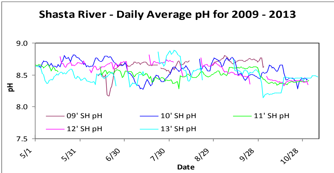
Figure 27. Daily average pH concentrations for the Shasta River from 2009-2013.
