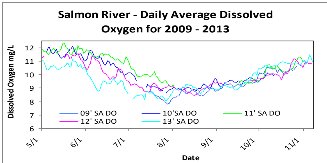
Figure 24. Daily average dissolved oxygen concentrations for the Salmon River from 2009-2013.
