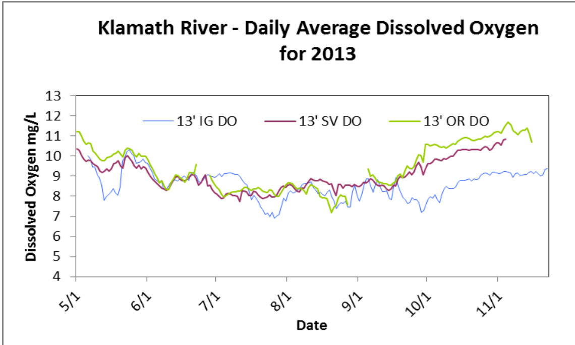
Figure 5. Daily average dissolved oxygen levels for 3 mainstem Klamath River sites in 2013: below Iron Gate dam (IG), Seiad Valley (SV), and Orleans (OR).
