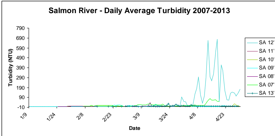
Figure 34 . Daily average turbidity, winters of 2007 - 2013 on Salmon River (SA).
