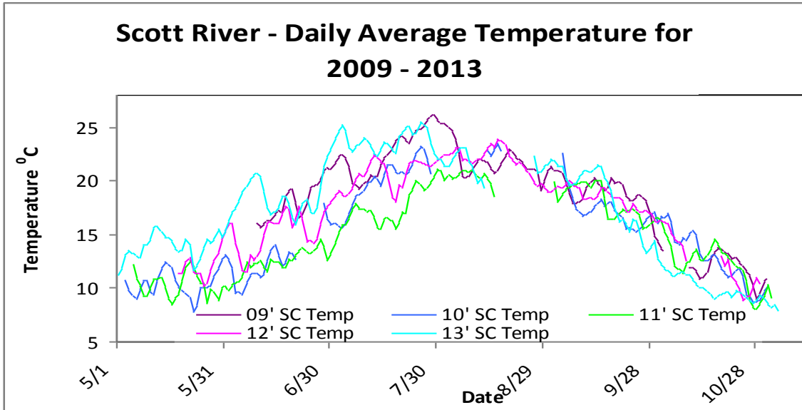
Figure 17. Daily average water temperatures for the Scott River from 2009-2013.
