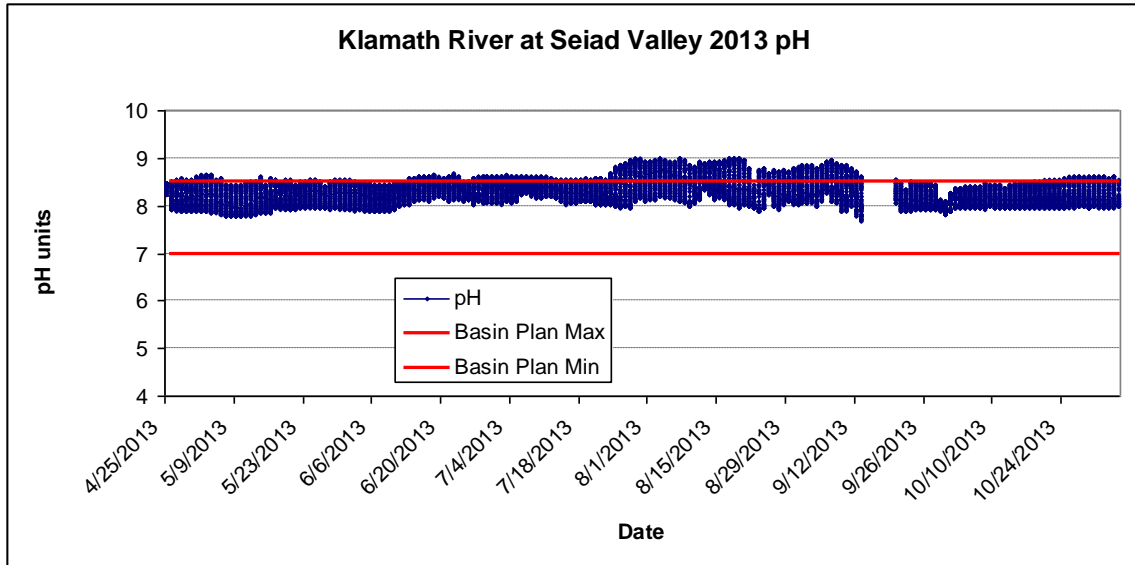
Figure 12. Instantaneous pH readings recorded every 30-minutes for Klamath River below Seiad Valley (SV) in 2013. The red lines are the NCRWQCB Basin Plan water quality objectives for the Klamath River, 7 < X < 8.5
