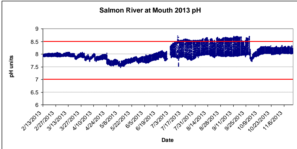
Figure 32. Instantaneous pH readings recorded every 30 minutes for the mouth of the Salmon River (SA) in 2013. The red line indicates the NCRWQCB Basin Plan pH water quality objective for Salmon River, 7 < X < 8.5 .
