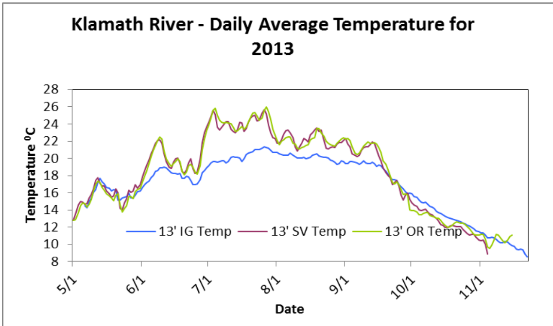
Figure 3. Daily average temperatures for 3 mainstem Klamath River sites in 2013: below Iron Gate dam (IG), Seiad Valley (SV), and Orleans (OR).
