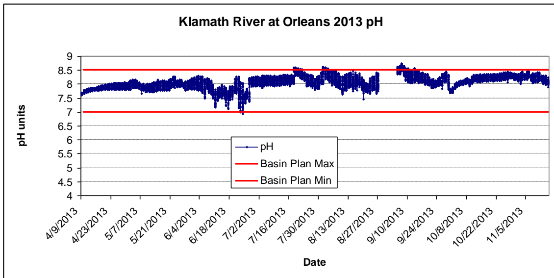
Figure 11. Instantaneous pH readings recorded every 30-minutes for Klamath River at Orleans (OR) in 2013. The red lines are the NCRWQCB Basin Plan water quality objectives for the Klamath River, 7 < X < 8.5 .
