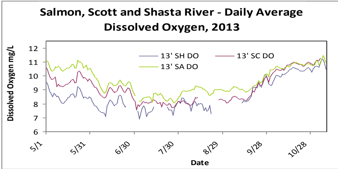
Figure 19. Daily average dissolved oxygen for Salmon, Scott and Shasta River, 2013.
