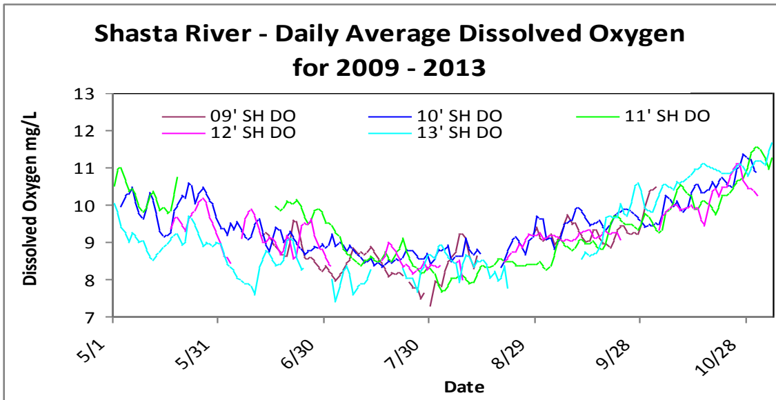
Figure 20. Daily average dissolved oxygen concentrations for the Shasta River from 2009-2013.
