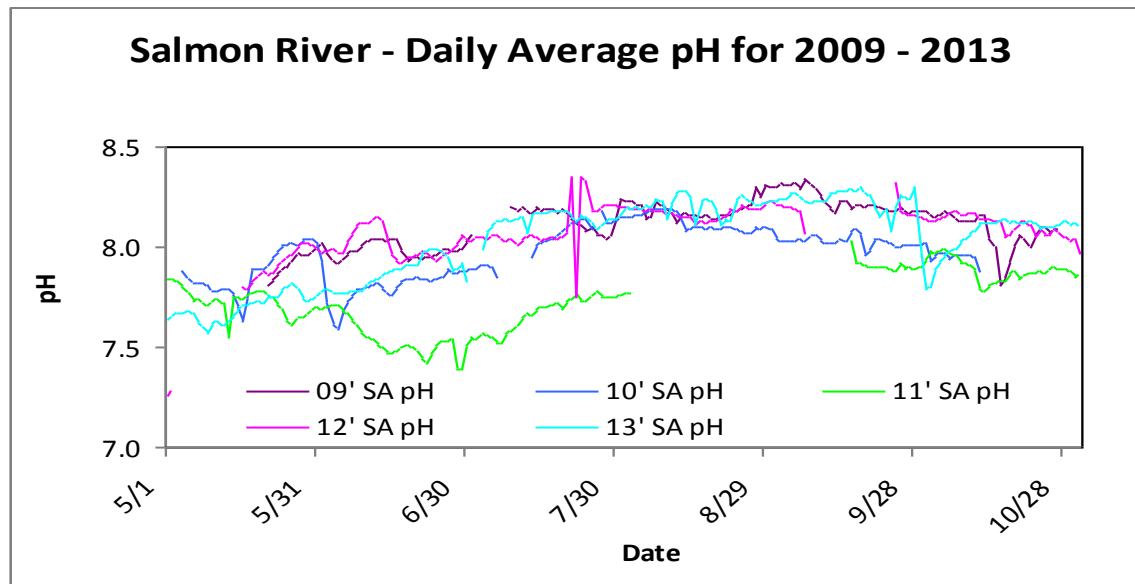
Figure 31. Daily average pH concentrations for the Salmon River from 2009-2013.
