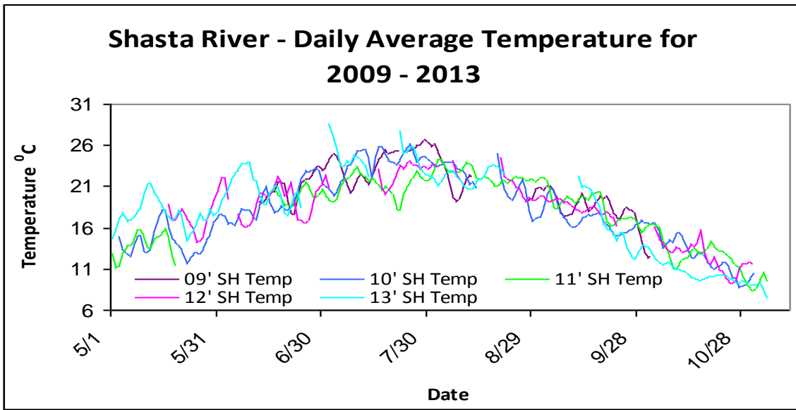
Figure 16. Daily average water temperatures for the Shasta River from 2009-2013.
