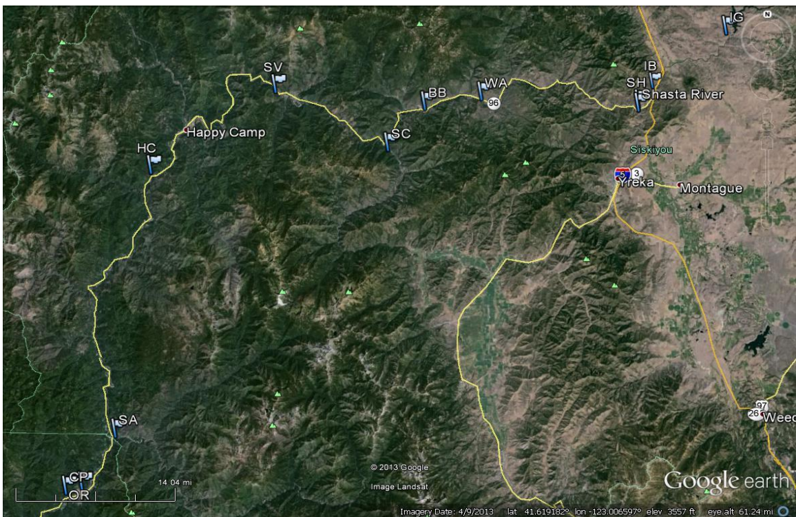
Figure 1. Overview of the Karuk Tribe’s water quality monitoring locations along the Klamath River in 2013.
