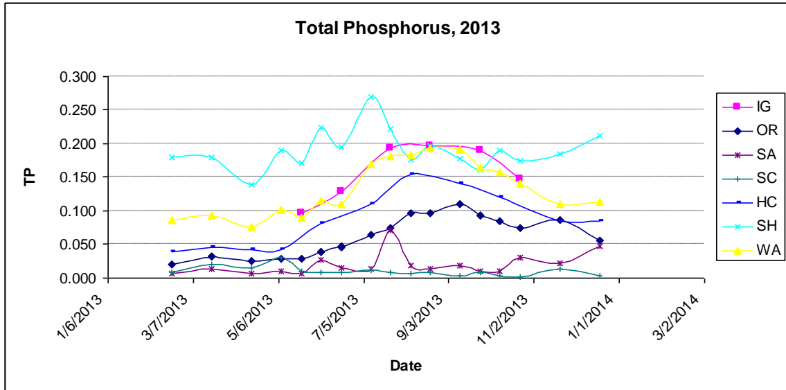
Figure 35. Total Phosphorus measured in mg/L for all monitored sites during 2013.
