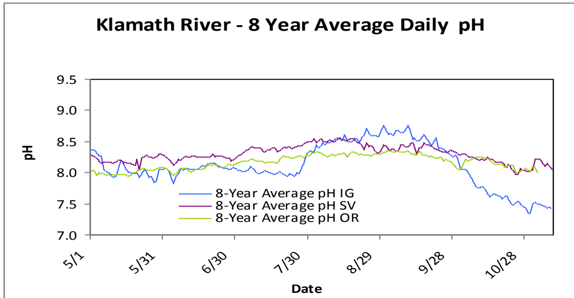
Figure 14. Daily average pH, 2006-2013 at mainstem Klamath River sites: below Iron Gate dam (IG), Seiad Valley (SV), and Orleans (OR).
