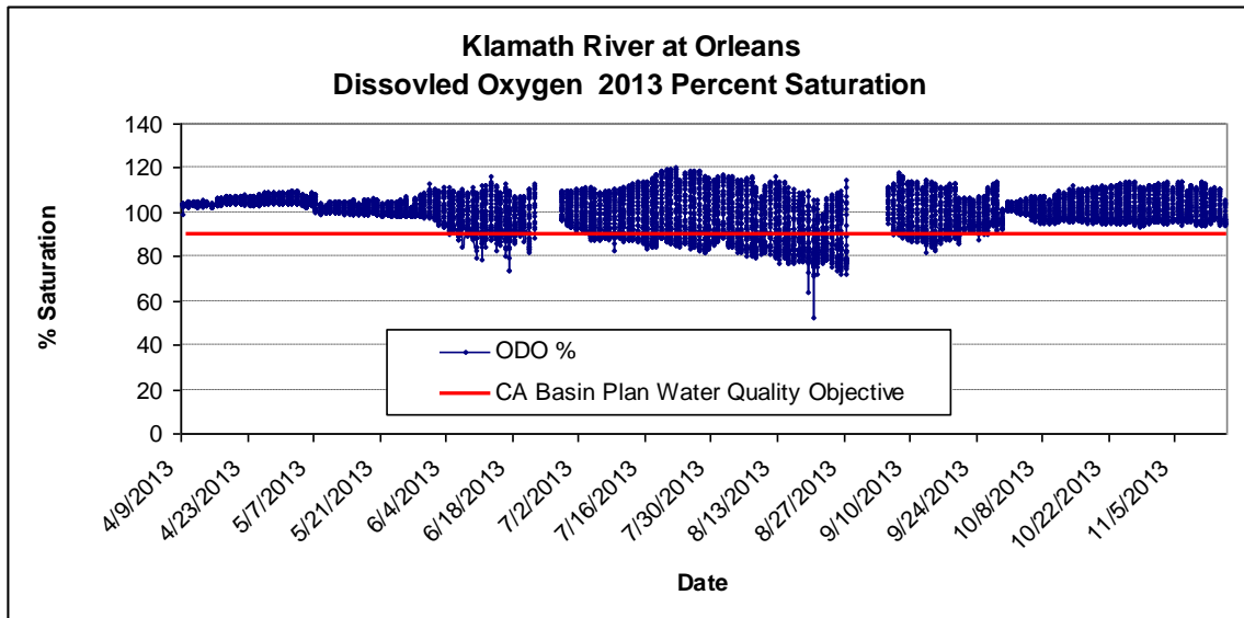
Figure 6. Percent saturation dissolved oxygen readings recorded every 30-minutes for Klamath River at Orleans (OR) in 2013. The red line indicates the NCRWQCB
